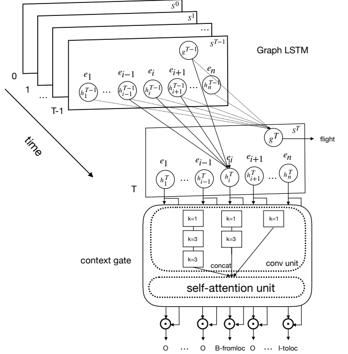
Figure 2: An overview of our proposed model. The Graph LSTM views the whole sentence as a single graph S and uses message passing mechanism to learn the node representation. After T time steps, we use the final word-level node h_i^T to predict the i_{th} slot label and the sentence-level node g^T to predict intent (where T is hyperparameter). For SF, a context gate, which consists of a convolution unit and a self-attention unit, is further added on top of the Graph LSTM to capture local and global context information.
